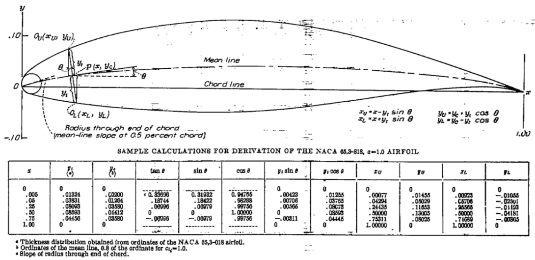
FIGURE 1.—Method of combining mean lines and basic thickness forms.
